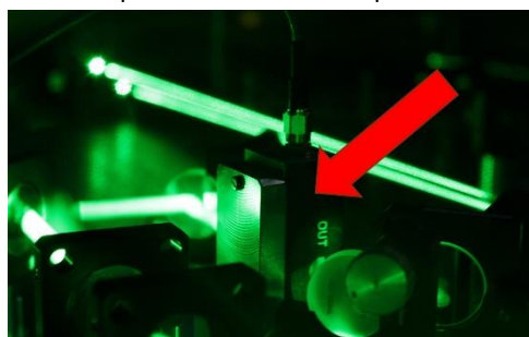
The Acousto-Optic Deflector (red arrow) splits one laser beam into many controllable single beams which catch and hold the atoms
