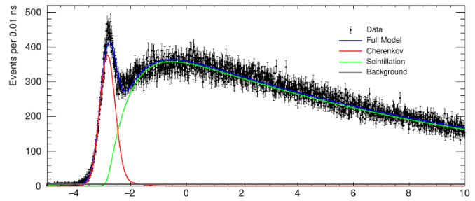
Typical light emission kinematics for a slow liquid scintillation mixture. The Cherenkov light (red line) in form of a sharp peak in time is followed by the slower scintillation light decay (green line)
